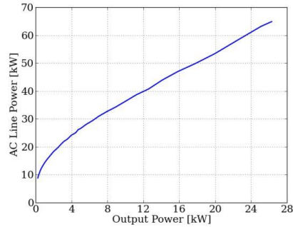
Figure 9: AC line power vs. output power.
