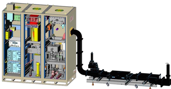
Figure 8: VIL410 cabinet layout and circulator.
