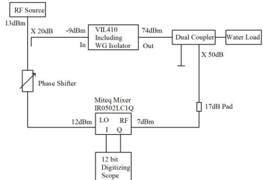
Figure 6: Measuring phase and amplitude ripple.
