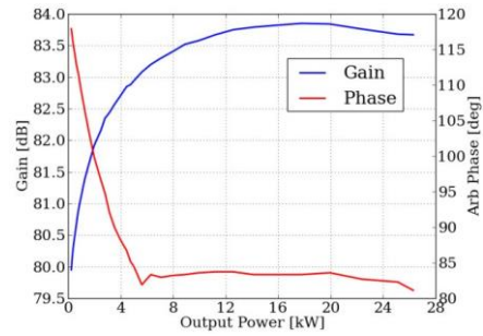
Figure 3: Gain and phase vs. output power.
